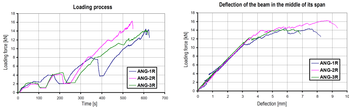
Fig. 2 Loading diagram of the reinforced glass beams (left) and diagrams of P - w relationship of the reinforced glass beams (right)
