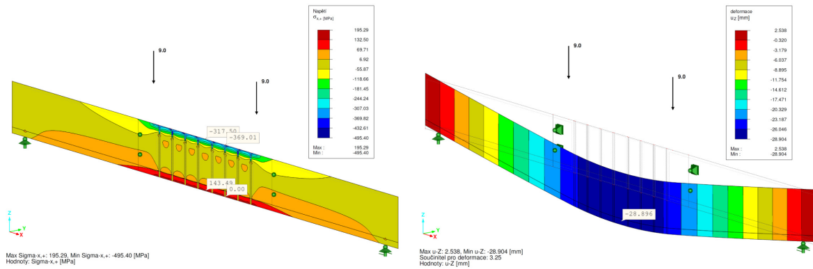
Fig. 6 Normal stress \sigma_{xx} in the glass and vertical deflection U_z for loading force P = 18\text{kN} eight crack, non-linear material model of the reinforcement
