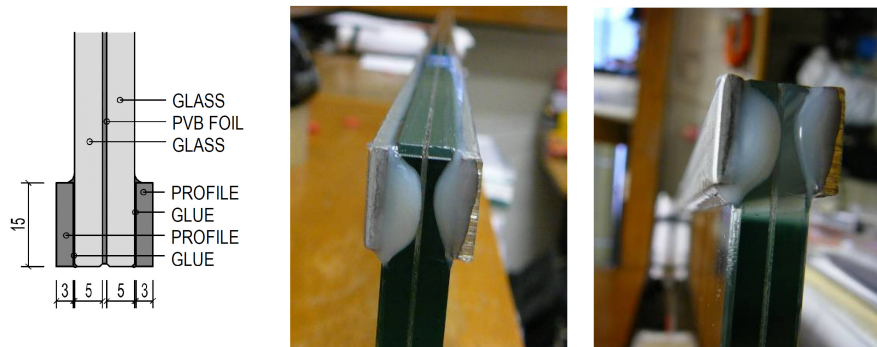
Fig. 1 Glued reinforcing profile (detail), scheme and the real performance
