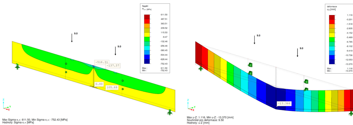
Fig. 5 Normal stress \sigma_x in the glass and vertical deflection U_z for loading force P = 18\text{kN} one crack, non-linear material model of the reinforcement
